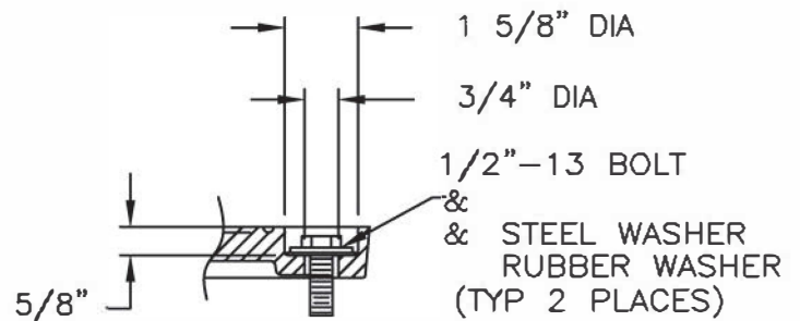
BOLTHOLE DETAIL
