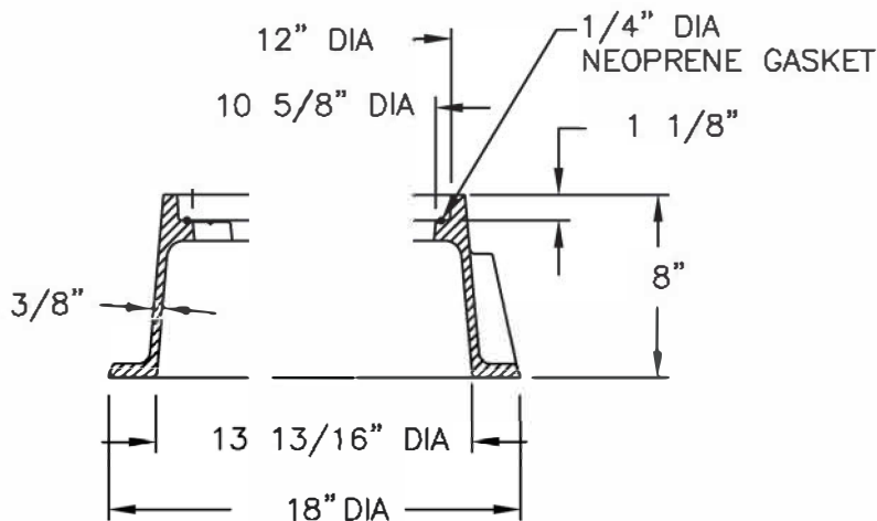
FRAME SECTION
