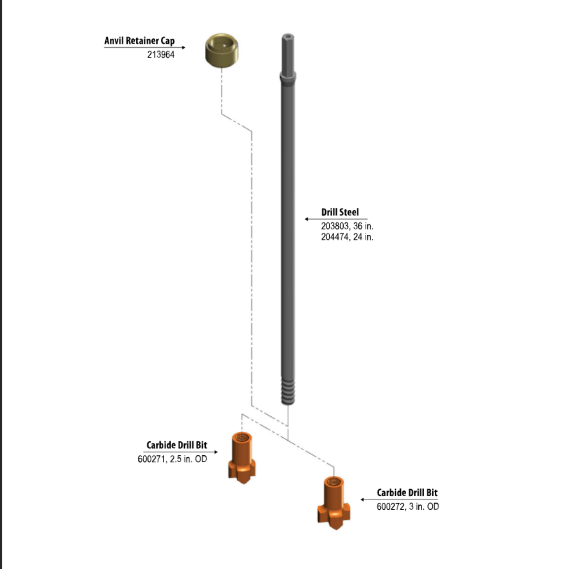
Tool String Diagram
